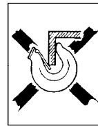
Fig 3 d Hook tip subject to additional bending stress
