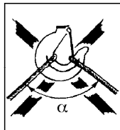
Fig 3 b Too great a top angle on the sling \alpha = \max 60^\circ
