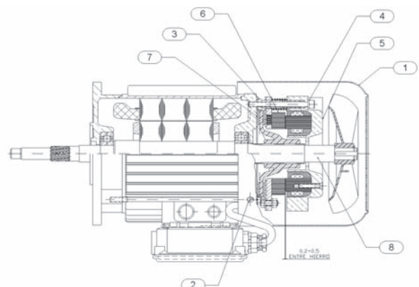
Figure 12, Two-speed Brake Motor, ABK201
