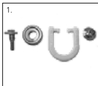
1. Constituent parts. Ensure that the locking ring is mounted on the bolt.
